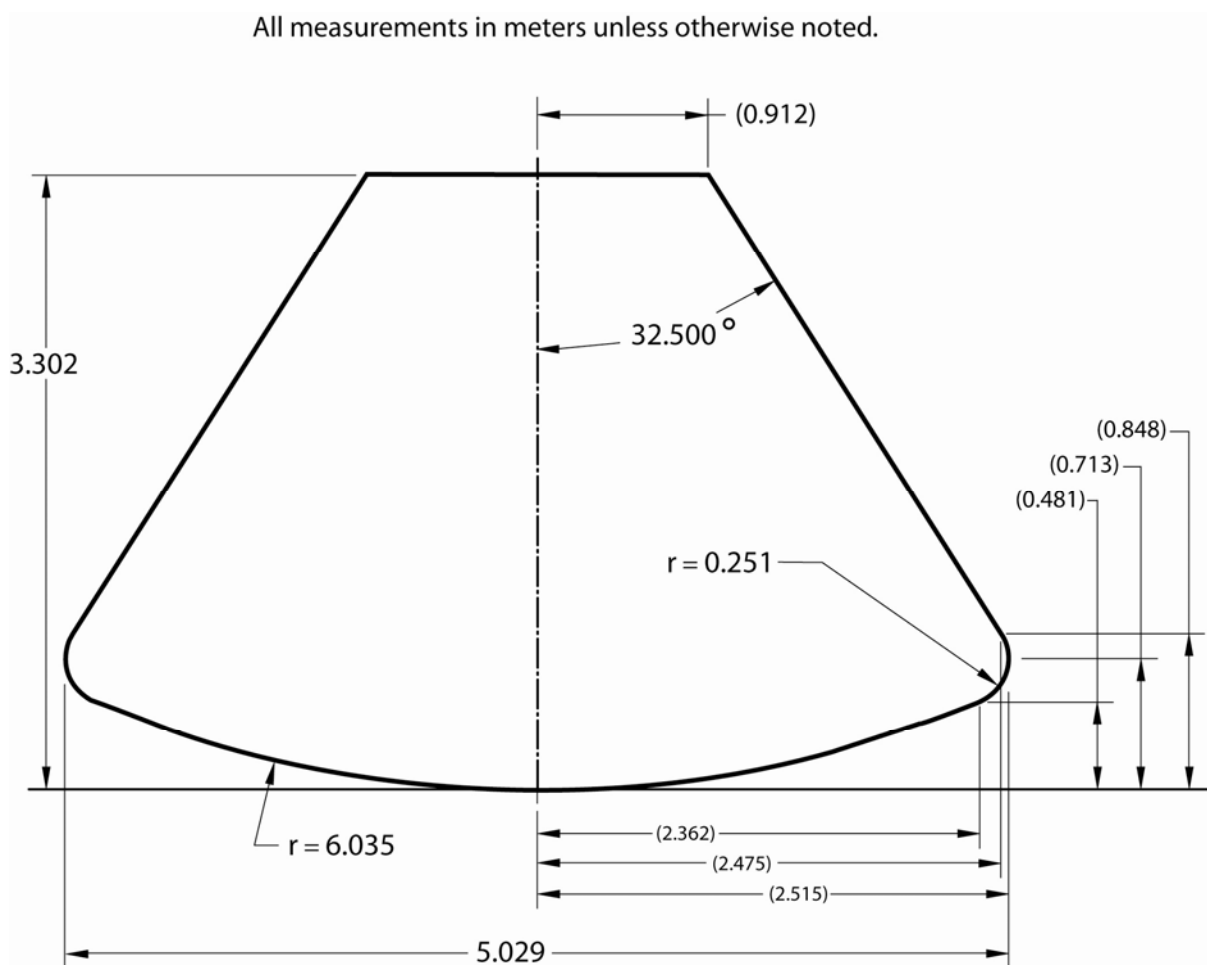
Figure 4: Largest vertical cross-section of the Orion crew module
