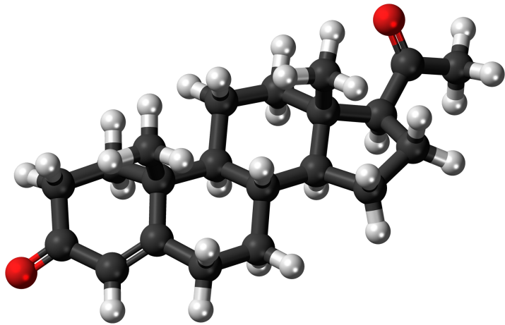
Progesterone molecule
