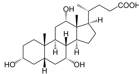
cholic acid
