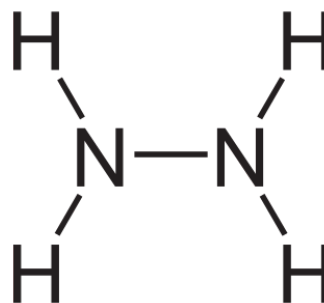
Hydrazine
