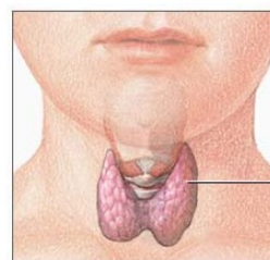
Thyroid gland
