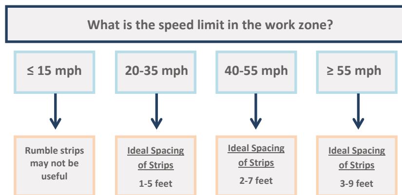
Figure 6. Recommended spacing of rumble strips based on work zone speed limit.
