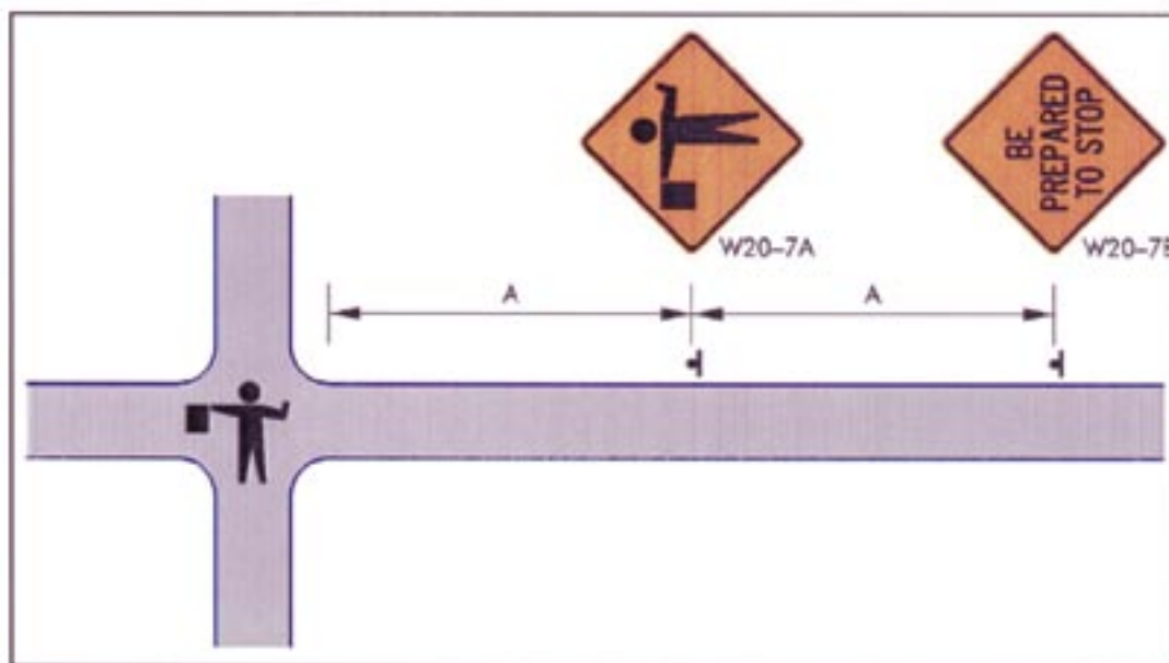
Figure 6-10. Standard signing plan for flagger-controlled intersection. (Source: Idaho Transportation Department)
